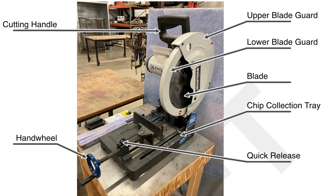
Figure 1: Annotated full view of the metal chop saw.
