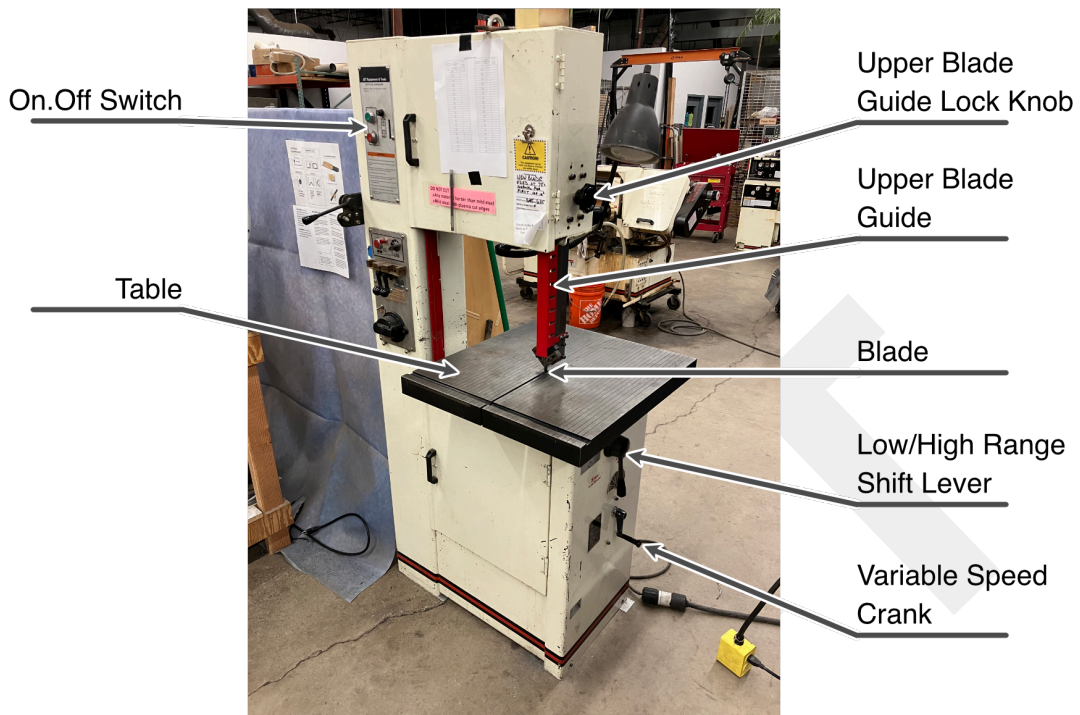
Figure 5: Annotated front quarter view of the vertical metal band saw.
