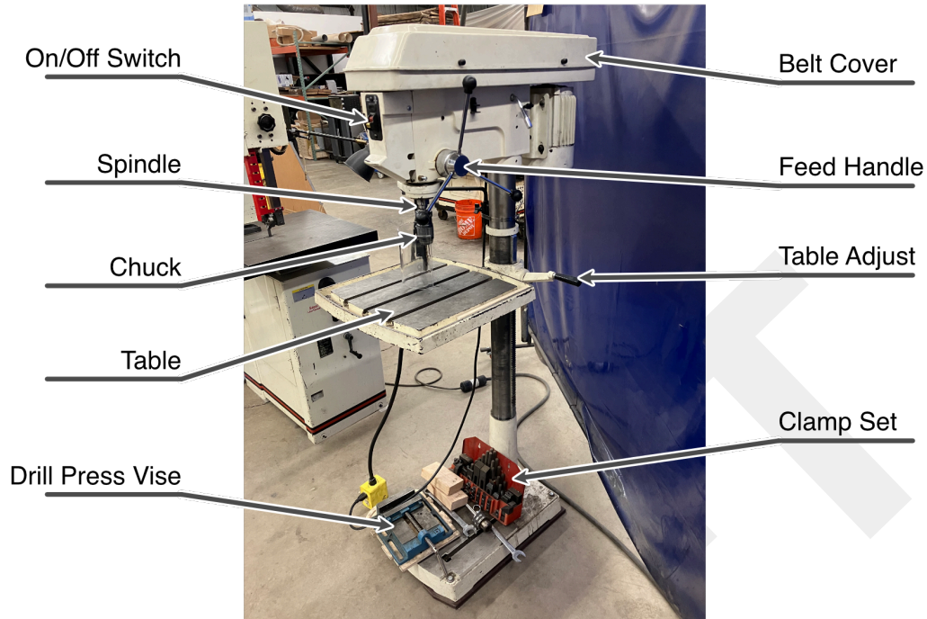
Figure 3: Annotated full view of the metal drill press.
