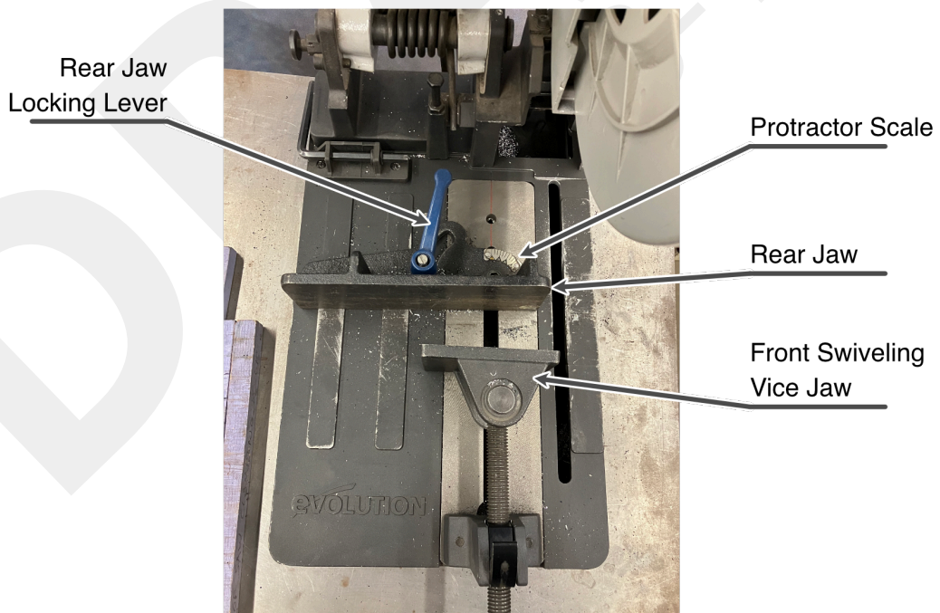
Figure 2: Annotated full view of the metal chop saw table.
